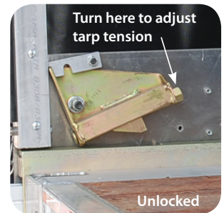
The adjustable rear lock gives you the ability to fine tune your tarp tension.
