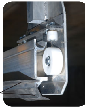
Dual mudguards are flexible enough to wrap around straps and chains and to keep road spray away from your load.
