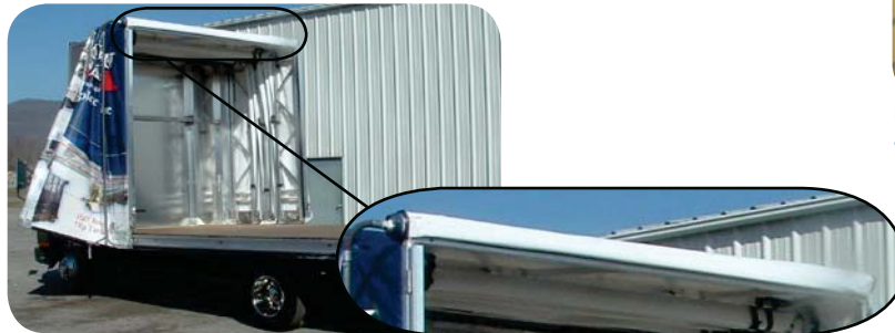
Retracted system showing rolled up rear door and the 100% height clearance that it provides.
